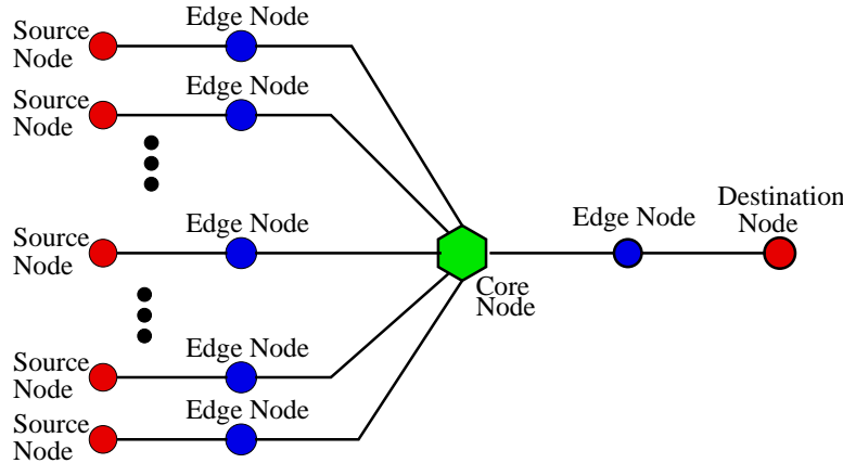
Figure 7.1: Network topology
