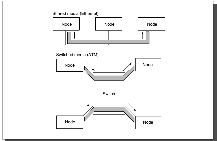
FIGURE 8.12 Shared medium versus switch. Ethernet was originally a shared medium, and but Ethernet switches are now available. All nodes on the shared media must share the 100 Mb/sec interconnection, but switches can support multiple 100 Mb/sec transfers simultaneously. Low cost Ethernet switches are sometimes implemented with an internal bus with higher bandwidth, but high-speed switches have a cross-bar interconnect.
