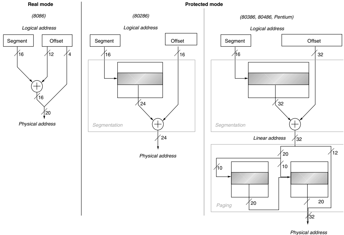
Figure D.3 The original segmented scheme of the 8086 is shown on the left. All 80x86 processors support this style of addressing, called real mode . It simply takes the contents of a segment register, shifts it left 4 bits, and adds it to the 16-bit offset, forming a 20-bit physical address. The 80286 (center) used the contents of the segment register to select a segment descriptor, which includes a 24-bit base address among other items. It is added to the 16-bit offset to form the 24-bit physical address. The 80386 and successors (right) expand this base address in the segment descriptor to 32 bits and also add an optional paging layer below segmentation. A 32-bit linear address is first formed from the segment and offset, and then this address is divided into two 10-bit fields and a 12-bit page offset. The first 10-bit field selects the entry in the first-level page table, and then this entry is used in combination with the second 10-bit field to access the second-level page table to select the upper 20 bits of the physical address. Prepending this 20-bit address to the final 12-bit field gives the 32-bit physical address. Paging can be turned off, redefining the 32-bit linear address as the physical address. Note that a “flat” 80x86 address space comes simply by loading the same value in all the segment registers; that is, it doesn’t matter which segment register is selected.
