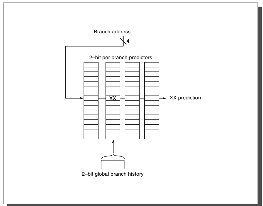
FIGURE 3.14 A (2,2) branch-prediction buffer uses a two-bit global history to choose from among four predictors for each branch address. Each predictor is in turn a two-bit predictor for that particular branch. The branch-prediction buffer shown here has a total of 64 entries; the branch address is used to choose four of these entries and the global history is used to choose one of the four. The two-bit global history can be implemented as a shifter register that simply shifts in the behavior of a branch as soon as it is known.
