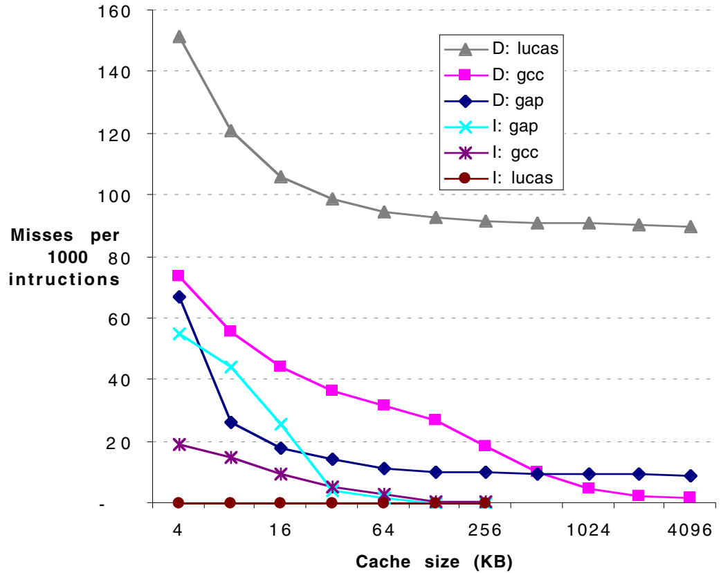
FIGURE 5.52 Instruction and data misses per thousand instructions for as cache size varies from 4 KB to 4096 KB. Instruction misses for gcc are 30,000 to 40,000 times larger than lucas, and conversely, data misses for lucas are 2 to 60 times larger than gcc. The programs gap, gcc, and lucas are from the SPEC2000 benchmark suite. These data are from the same experiment as in Figure 5.10.
