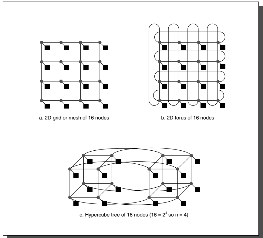
FIGURE 8.16 Network topologies that have appeared in commercial supercomputers.
