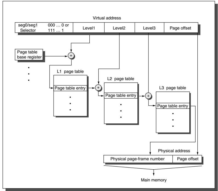
FIGURE 5.39 The mapping of an Alpha virtual address. This figure/description shows the 21264's virtual memory implementation with 3 page table levels, which supports an effective physical address size of 41 bits (allowing access up to 2^{40} bytes of memory and 2^{40} I/O addresses). Each page table is exactly one page long, so each level field is n bits wide where 2^n = \text{page size}/8 . The Alpha architecture document allows the page size to grow from 8 KB in the current implementations to 16 KB, 32 KB, or 64 KB in the future. The virtual address for each page size grows from the original 43 bits to 47, 51, or 55 bits and the maximum physical address size grows from the current 41 bits to 45, 47, or 48 bits. The 21264 also can support a 4-level page table structure (with a level 0 page table field in virtual address bits 43-52) that can allow full access to its 44-bit physical address and 48-bit virtual address while keeping page sizes to 8 KB. That mode is not depicted here. In addition, the size depends on the operating system. VMS does not require KSEG like UNIX does, so VMS could reach the entire 44-bit physical address space with 3-level page tables. The 41-bit physical address restriction comes from the fact that some operating systems need the KSEG section.
