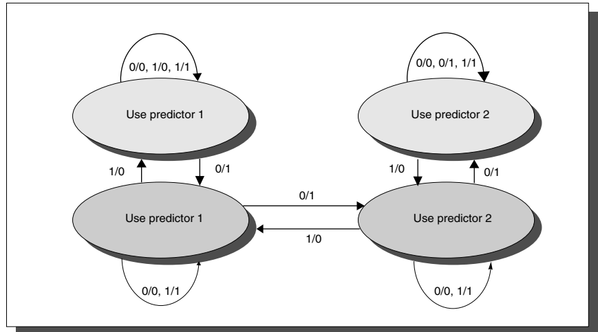
FIGURE 3.16 The state transition diagram for a tournament predictor has four states corresponding to which predictor to use. The counter is incremented whenever the “predicted” predictor is correct and the other predictor is incorrect, and it is decremented in the reverse situation.
