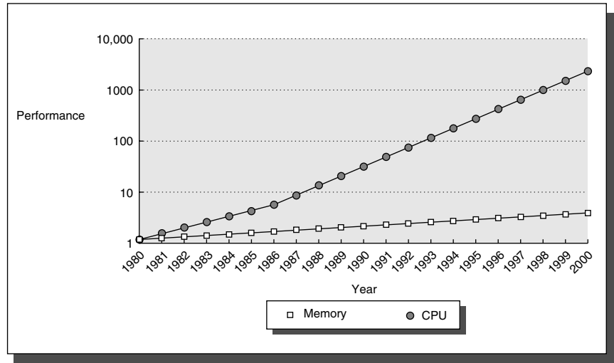
FIGURE 5.2 Starting with 1980 performance as a baseline, the gap in performance between memory and CPUs are plotted over time. Note that the vertical axis must be on a logarithmic scale to record the size of the CPU-DRAM performance gap. The memory baseline is 64-KB DRAM in 1980, with three years to the next generation and a 7% per year performance improvement in latency (see Figure 5.30 on page 444). The CPU line assumes a 1.35 improvement per year until 1986, and a 1.55 improvement thereafter. <<NOTE: Artist continue the X-axis to 2005: DRAM should be 5.4 in 2005, and CPU should be 25,000 in 2005. This means the Y-axis needs to be extended to 100,000 to accommodate.>>
