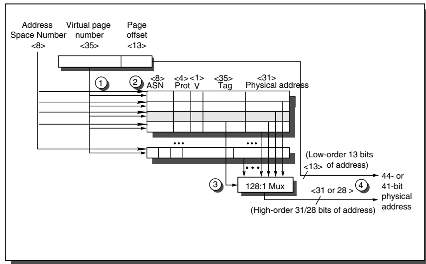
FIGURE 5.36 Operation of the Alpha 21264 data TLB during address translation. The four steps of a TLB hit are shown as circled numbers. The Address Space Number (ASN) is used like a Process ID for virtual caches, in that the TLB is not flushed on a context switch, only when ASNs are recycled. The next fields of an entry are protection permissions (Prot) and the valid bit (V). Note that there is no specific reference, use bit, or dirty bit. Hence, a page replacement algorithm such as LRU must rely on disabling reads and writes occasionally to record reads and writes to pages to measure usage and whether or not pages are dirty. The advantage of these omissions is that the TLB need not be written during normal memory accesses nor during a TLB miss. Alpha 21264 has an option of either 44-bit or 41-bit physical addresses. This TLB has 128 entries.
