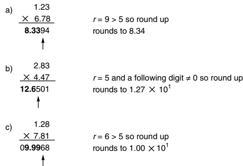
Figure H.9 Examples of rounding a multiplication. Using base 10 and p = 3 , parts (a) and (b) illustrate that the result of a multiplication can have either 2p - 1 or 2p digits, and hence the position where a 1 is added when rounding up (just left of the arrow) can vary. Part (c) shows that rounding up can cause a carry-out.
