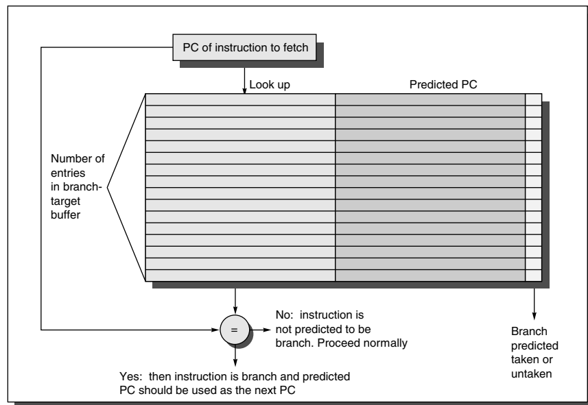
FIGURE 3.19 A branch-target buffer. The PC of the instruction being fetched is matched against a set of instruction addresses stored in the first column; these represent the addresses of known branches. If the PC matches one of these entries, then the instruction being fetched is a taken branch, and the second field, predicted PC, contains the prediction for the next PC after the branch. Fetching begins immediately at that address. The third field, which is optional, may be used for extra prediction state bits.
