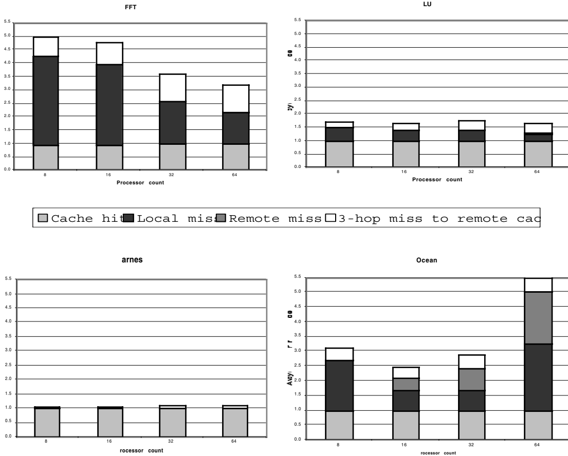
FIGURE 6.36 The effective latency of memory references in a DSM multiprocessor depends both on the relative frequency of cache misses and on the location of the memory where the accesses are served. These plots show the memory access cost (a metric called average memory access time in Chapter 5) for each of the benchmarks for 8, 16, 32, and 64 processors, assuming a 512KB data cache that is two-way set associative with 64-byte blocks. The average memory access cost is composed of four different types of accesses, with the cost of each type given in Figure 6.35. For the Barnes and LU benchmarks, the low miss rates lead to low overall access times. In FFT, the higher access cost is determined by a higher local miss rate (1-4%) and a significant 3-hop miss rate (1%). The improvement in FFT comes from the reduction in local miss rate from 4% to 1%, as the aggregate cache increases. Ocean shows the biggest change in the cost of memory accesses, and the highest overall cost at 64 processors. The high cost is driven primarily by a high local miss rate (average 1.6%). The memory access cost drops from 8 to 16 processors as the grids more easily fit in the individual caches. At 64 processors, the data set size is too small to map properly and both local misses and coherence misses rise, as we saw in Figure 6.31.
