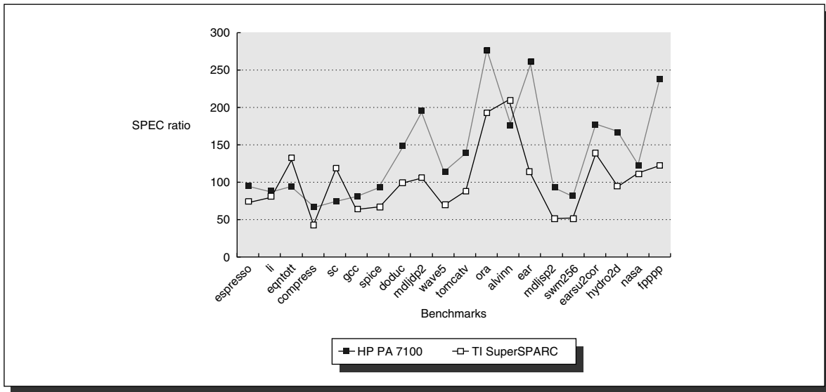
FIGURE 3.59 The performance of a 99-MHz HP PA 7100 processor versus a 60-MHz SuperSPARC. The comparison is based on 1994 measurements.
