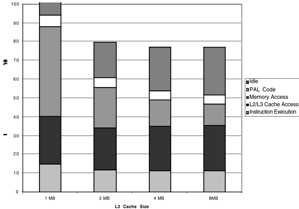
FIGURE 6.14 The relative performance of the OLTP workload as the size of the L3 cache, which is set as 2-way set associative, is grown from 1 MB to 8MB. Interestingly, the performance of the 1 MB, 2-way set associative cache is very similar to the direct-mapped 2 MB cache that is used in the Alphaserver 4100.
