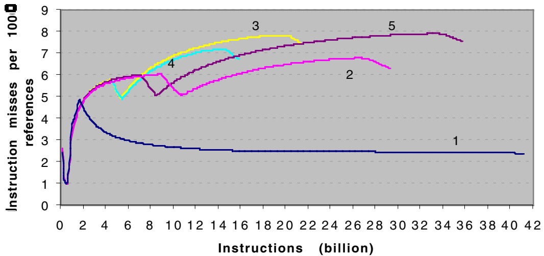
FIGURE 5.53 Instruction misses per 1000 references for five inputs to perl benchmark from SPEC2000. There is little variation in misses and little difference between the five inputs for the first 1.9 billion instructions, but running to completion shows how misses vary over the life of the program and how they depend on the input. The top graph shows the running average misses for the first 1.9 billion instructions, which starts at about 2.5 and ends at about 4.7 misses per 1000 references for all five inputs. The bottom graph shows the running average misses to run to completion, which takes 16 to 41 billion instructions depending on the input. After the first 1.9 billion instructions, the misses per 1000 references vary from 2.4 to 7.9 depending on the input. The simulations were for the Alpha processor using separate L1 caches for instructions and data, each 2-way 64KB with LRU, and a unified 1MB direct-mapped L2 cache.
