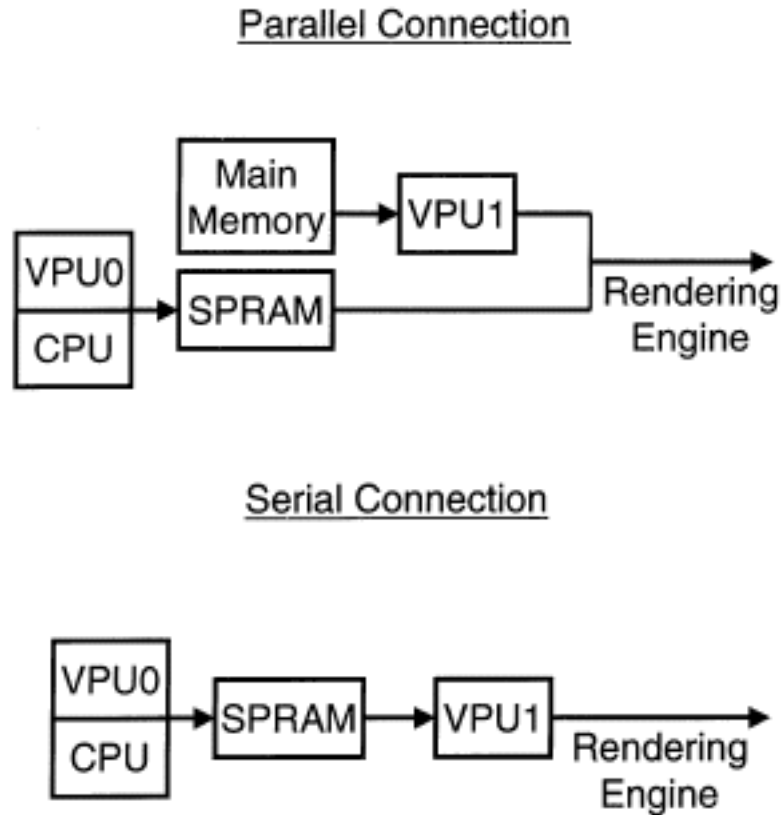
FIGURE 5.48 Two modes of using Emotion Engine organization. The first mode divides the work between the two units, and then allows the Graphics Interface to properly merge the display lists. The second more uses CPU/VPU0 as a filter of what to send to VPU1, which then does all the display lists. Its up to the programmer to chose between serial and parallel data flow. SPRAM is the scratchpad memory. <<Redraw with Serial on top, Parallel on Bottom; can be much smaller>>
