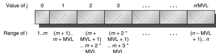
Figure G.8 A vector of arbitrary length processed with strip mining. All blocks but the first are of length MVL, utilizing the full power of the vector processor. In this figure, the variable m is used for the expression (n \bmod \text{MVL}) .
