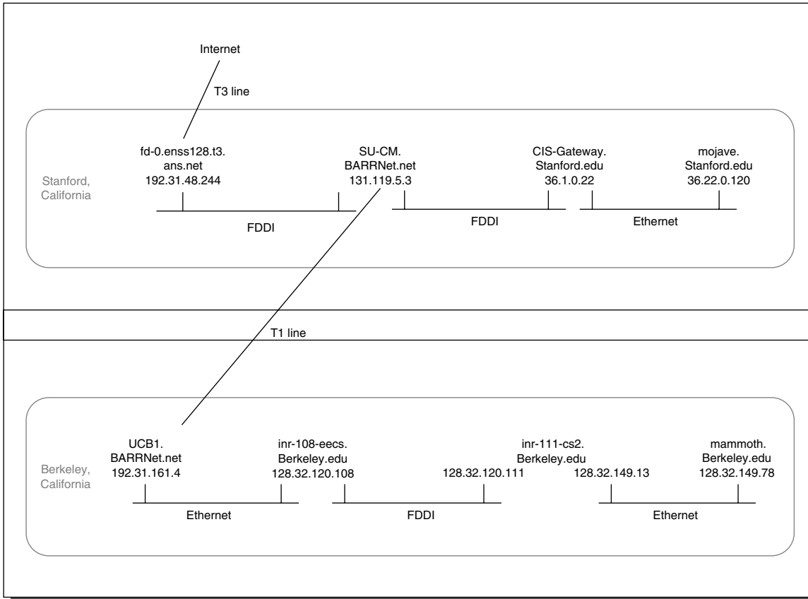
FIGURE 8.23 The connection established between mojave.stanford.edu and mammoth.berkeley.edu . (1995) FDDI is a 100 Mb/s LAN, while a T1 line is a 1.5 Mb/s telecommunications line and a T3 is a 45 Mb/s telecommunications line. BARRNet stands for Bay Area Research Network. Note that inr-111-cs2.Berkeley.edu is a router with two Internet addresses, one for each port.
