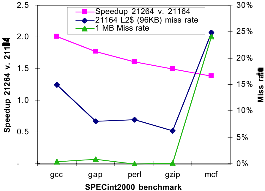
FIGURE 5.44 Alpha 21264/21164 Performance speedup vs. miss rates for SPECint2000. The left axis shows the speedup of the out-of-order 21264 is greatest with the highest miss rate of the 21164 L2 cache (right axis) as long as the access is a hit in the 21264 L2 cache. If it misses the L2 cache of the 21264, out-of-order execution is not as helpful. The 21264 is running at 500 MHz and the earlier 21164 is running at 533MHz.
