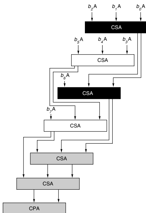
Figure H.29 Even/odd array. The first two adders work in parallel. Their results are fed into the third and fourth adders, which also work in parallel, and so on.
