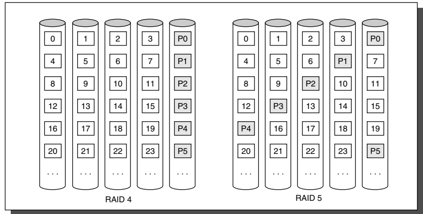
FIGURE 7.19 Block-interleaved parity (RAID 4) versus distributed block-interleaved parity (RAID 5). By distributing parity blocks to all disks, some small writes can be performed in parallel.
