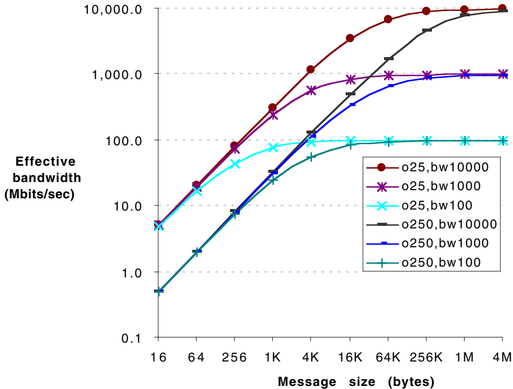
FIGURE 8.8 Bandwidth delivered versus message size for overheads of 25 and 250 microseconds and for network bandwidths of 100, 1000, and 10000 Mbits/second. Note that with 250 microseconds of overhead and a network bandwidth of 1000 Mbits/second, only the 4-MB message size gets an effective bandwidth of 1000 Mbits/second. In fact, message sizes must be greater than 256 B for the effective bandwidth to exceed 10 Mbits/second. The notation “oX,bwY” means an overhead of X microseconds and a network bandwidth of Y Mbits/second. <<Artist: label lines, drop legend.>>
