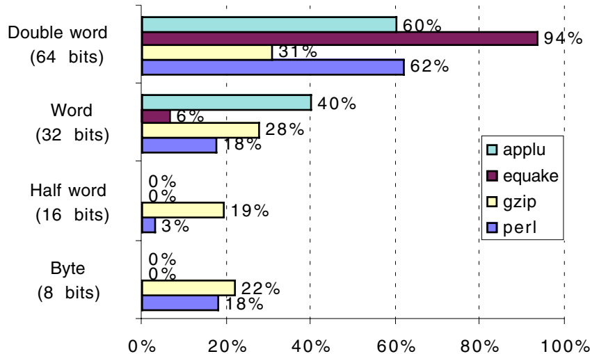
FIGURE 2.12 Distribution of data accesses by size for the benchmark programs. The double word data type is used for double-precision floating-point in floating-point programs and for addresses, since the computer uses 64-bit addresses. On a 32-bit address computer the 64-bit addresses would be replaced by 32-bit addresses, and so almost all double-word accesses in integer programs would become single word accesses.
