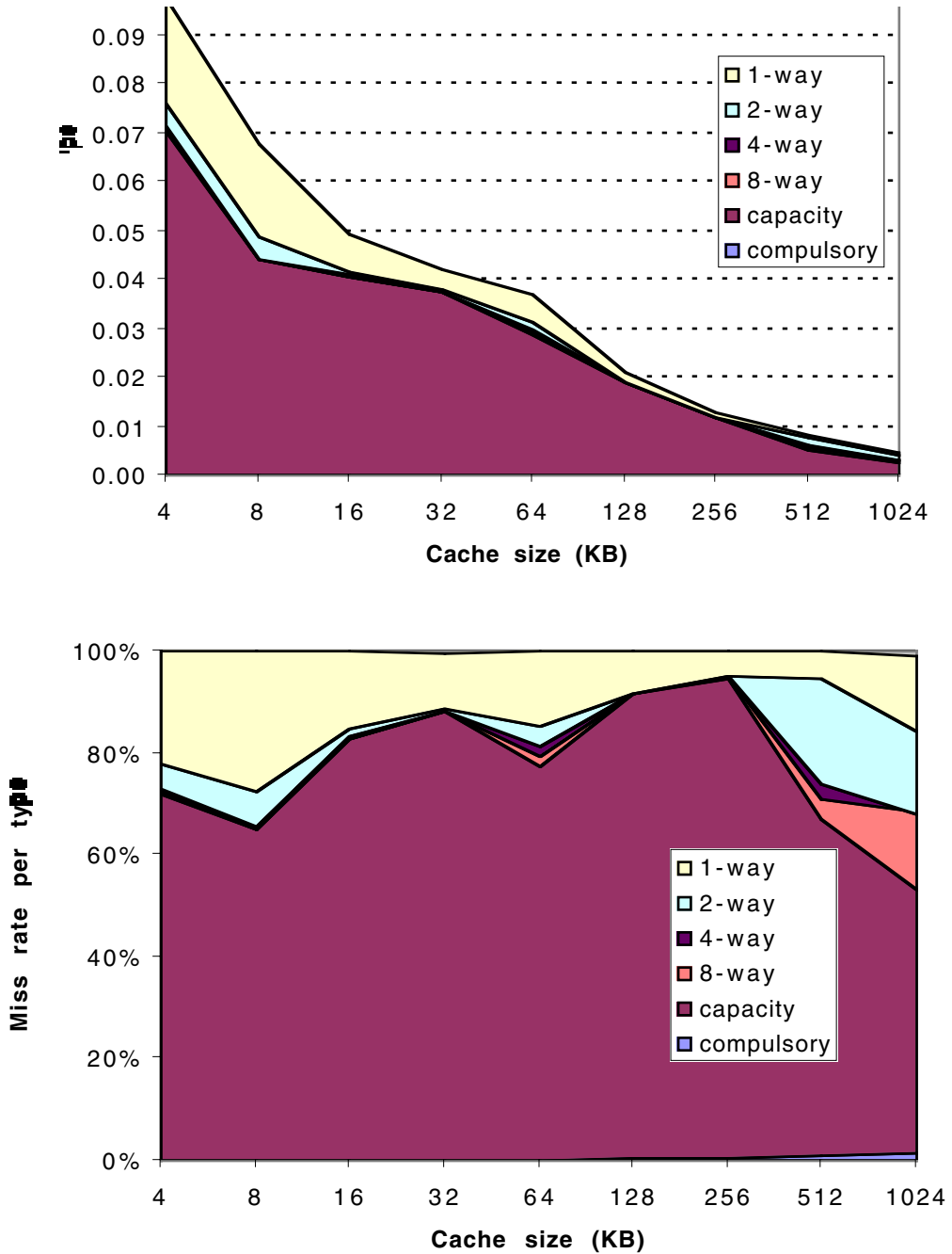
FIGURE 5.15 Total miss rate (top) and distribution of miss rate (bottom) for each size cache according to three C's for the data in Figure 5.14. The top diagram is the actual D-cache miss rates, while the bottom diagram shows percentage in each category. (Space allows the graphs to show one extra cache size than can fit in Figure 5.14.)
