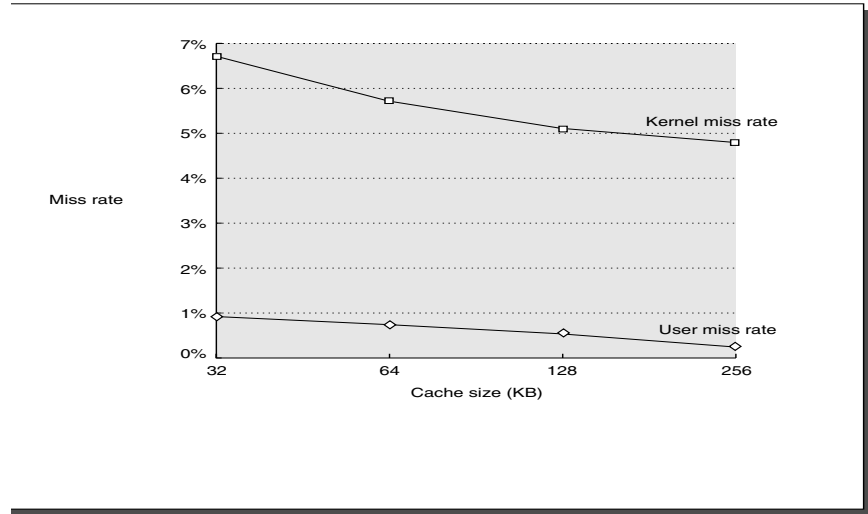
FIGURE 6.18 The data miss rate drops faster for the user code than for the kernel code as the data cache is increased from 32 KB to 256 KB with a 32-byte block. Although the user level miss rate drops by a factor of 3, the kernel level miss rate drops only by a factor of 1.3. As Figure 6.19 shows, this is due to a higher rate of compulsory misses and coherence misses. This multiprogramming workload is run on eight processors.
