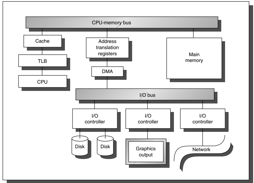
FIGURE 7.35 Virtual DMA requires a register for each page to be transferred in the DMA controller, showing the protection bits and the physical page corresponding to each virtual page.
